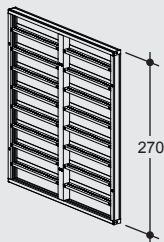
MANTO Großtafel 240/270 MANTO giant panel 240/270
