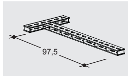
Eckkupplung H 20/R 24 Corner connector H 20/R 24
