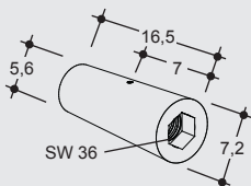
Ankerkonus M36 DW26,5 Tie cone M36 DW26.5
