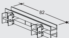
Ankerfurt Tie waler
