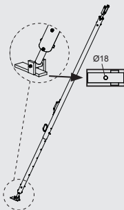
Richtstrebe K440 Aligning strut K440 Richtstrebe K600 Aligning strut K600 Richtstrebe K760 Aligning strut K760
