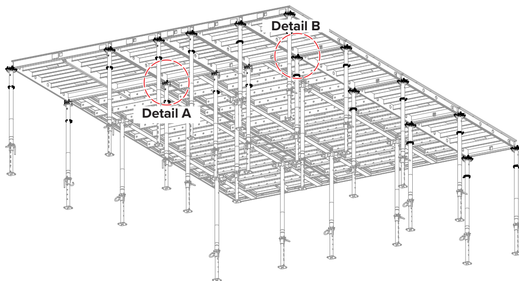
Detail A TOPMAX an TOPEC
