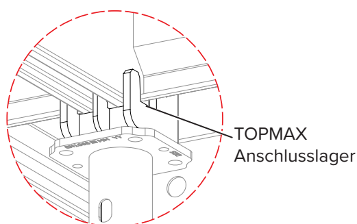
Detail A TOPMAX an TOPEC
