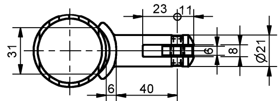
Detail Z
