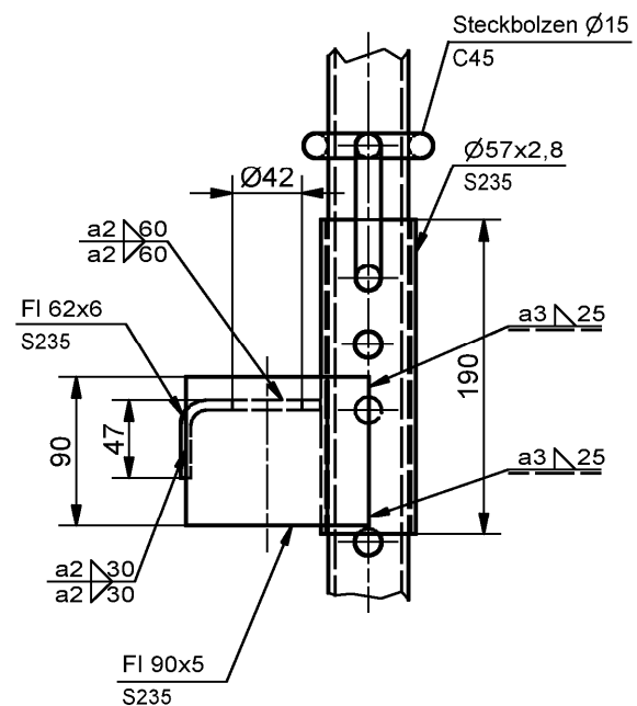
Detail X
