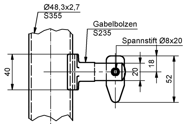
Detail Z
