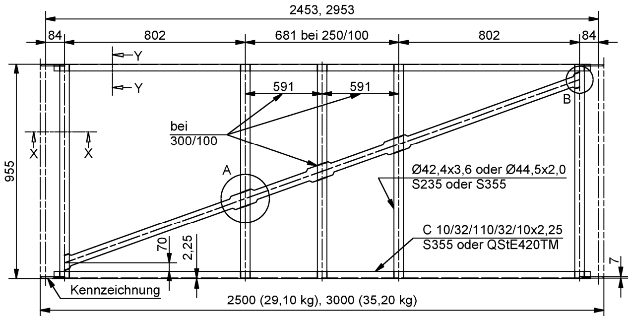
Detail A
