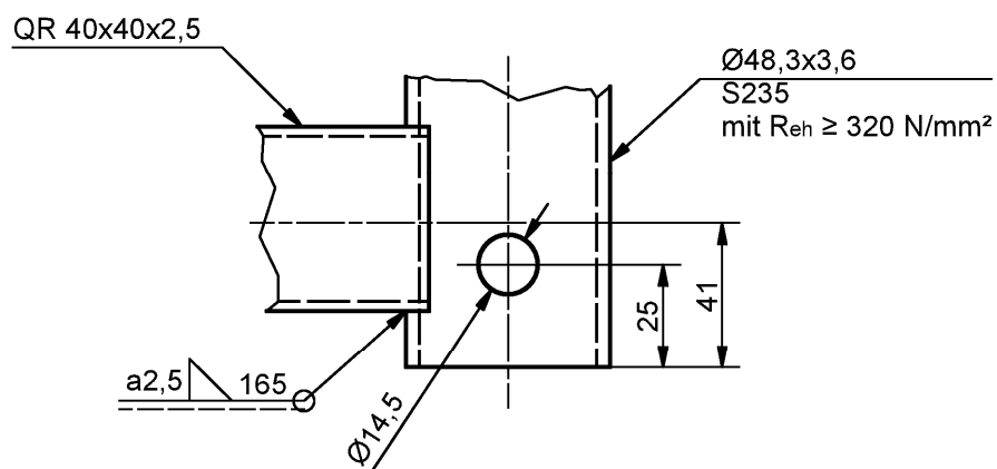
Detail W
